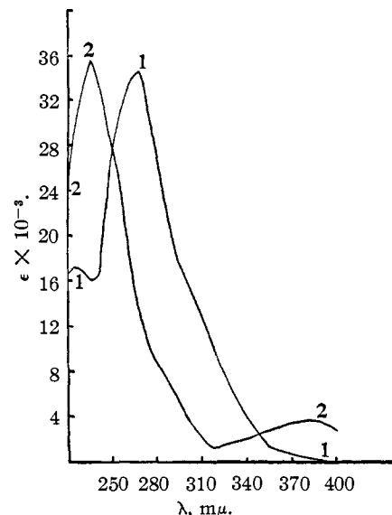
Fig. 3.—Absorption spectra of: m -nitroacetophenonazine, 1; diacetyldi-( m -nitroanil), 2.
